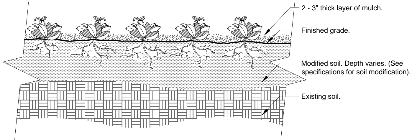
SECTION VIEW
